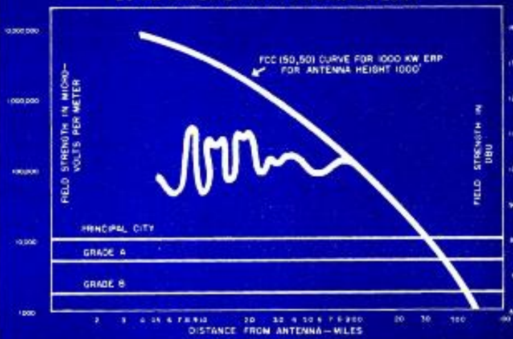
CALCULATED COVERAGE CURVE FOR OBTAINING 1000 KW ERP 23 KW AMPLIFIER WITH 50 GAIN ANTENNA
