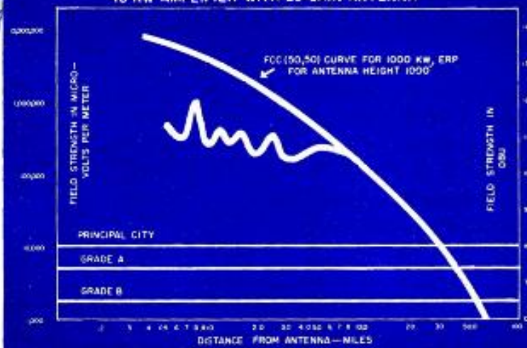
CALCULATED COVERAGE CURVE FOR OBTAINING 1000 KW ERP 45 KW AMPLIFIER WITH 25 GAIN ANTENNA
