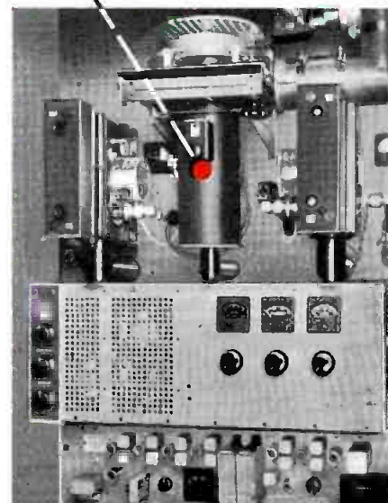
RCA-6181 tube and cavity in the driver stage of the aural section of WKBN-TV's 12½-KW UHF transmitter.
